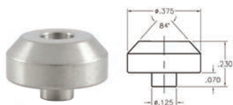
Standard Nozzle Assembly Diamond Sapphire
