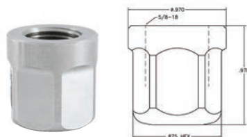
IDNN-HP (Integral Diamond Nozzle Nut) Diamond
