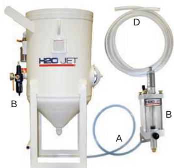
Abrasive Feed Kit Bulk Hopper, Gravity Meter & Feed Hose
