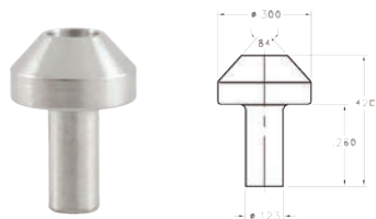
LM-II-L Nozzle Assembly Diamond Sapphire
